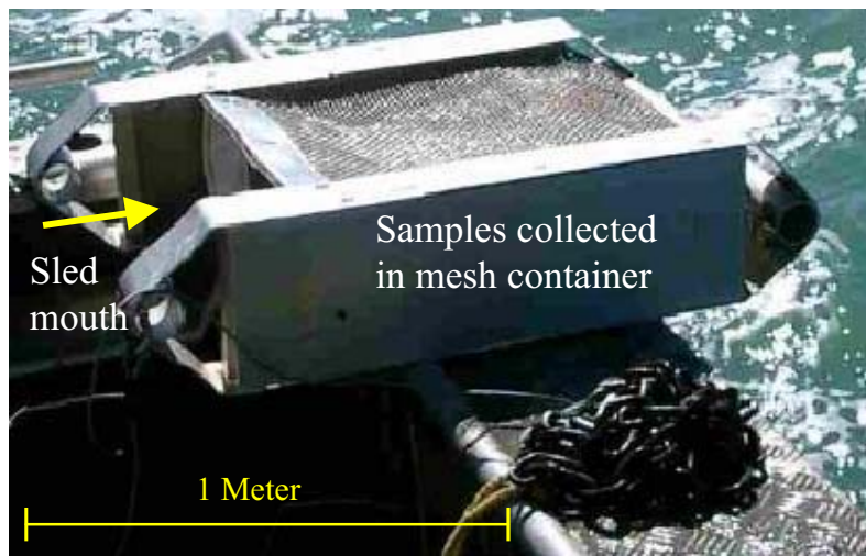
Figure 5: Benthic sled
