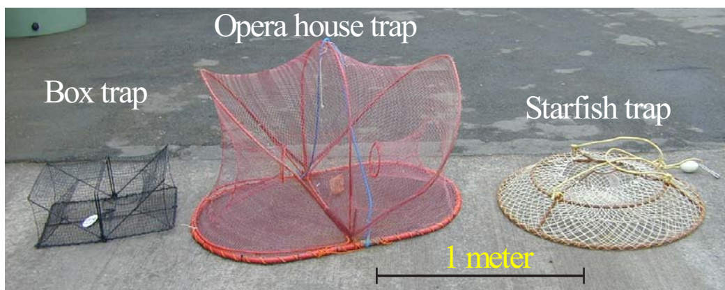
Figure 7: Trap types deployed in the port.
