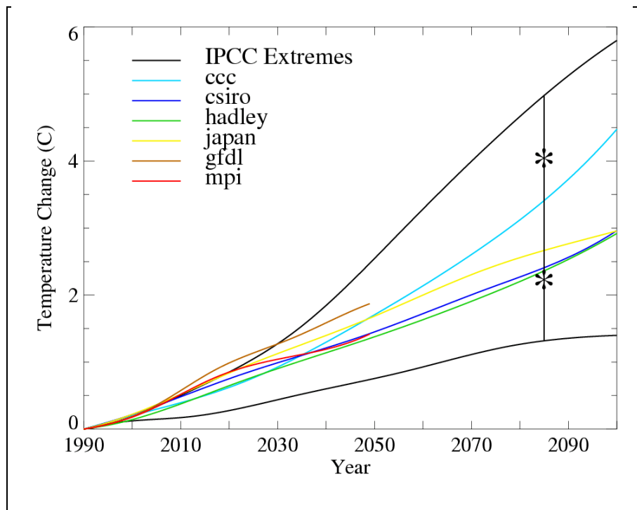
Figure 6.6.1 Global-mean surface temperature changes from a range of models (coloured lines), and the IPCC extreme range (black lines). Stars on the vertical bar at 2085 indicate schematically the IPCC 25 percentile and 75 percentile for the 2080s. Note that in practice (see text) we use a 30-year period, not a single year, and calculate the quartiles of the extreme low to high scaling factor range, not quartiles of the temperature change.
