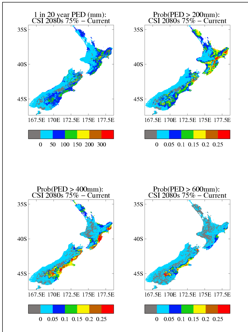
Figure 6.9.3 Change in drought statistics from the present for the CSIRO 2080s 75% scenario.
