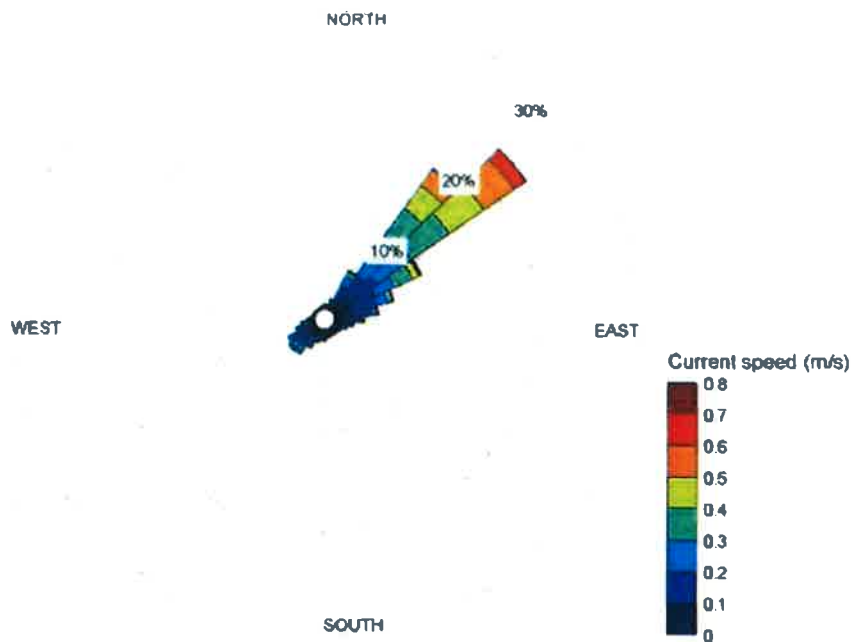
Figure No 2 Current rose showing current directions and magnitudes for the top four bins at mid Waitata Reach
