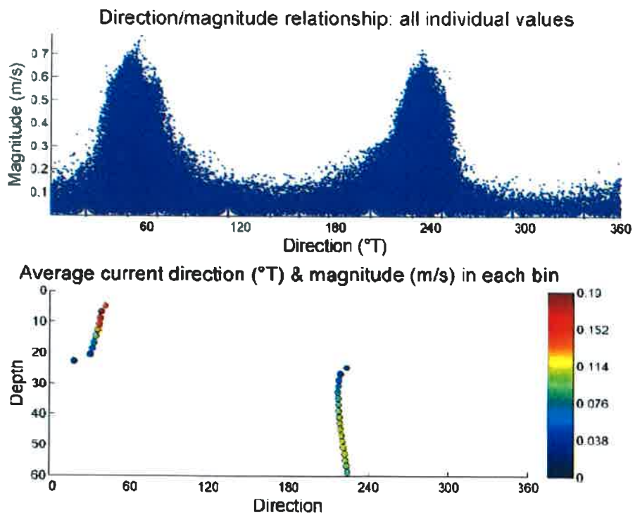
Figure No 4 All observations of current magnitude and direction (top panel) and time averaged profile magnitude and direction (bottom panel) at mid Waitata Reach
