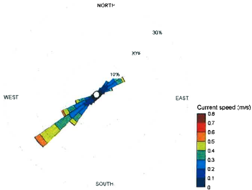
Figure No 3 Current rose showing current directions and magnitudes for the lowest four bins at mid Waitata Reach
