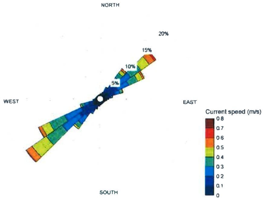
Figure No 1 Current rose showing current directions and magnitudes for all bins at mid Waitata Reach
