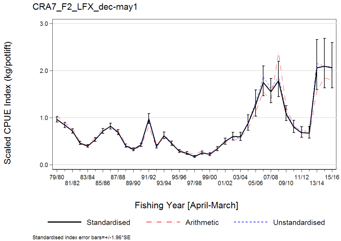
Figure 22: Annual CPUE indices for CRA 7: arithmetic (dashed line), unstandardised (dotted line), and standardised (bold line) \pm 1.96 s.e. from 1979–80 to 2015–16. The geometric mean for each series = 0.65 kg/potlift. This figure generated from data prepared using the F2 algorithm scaled to the combined “LFX” destination codes.
