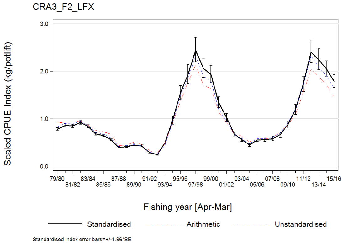
Figure 10: Annual CPUE indices for CRA 3: arithmetic (dashed line), unstandardised (dotted line), and standardised (bold line) \pm 1.96 s.e. from 1979–80 to 2015–16. The geometric mean for each series = 0.86 kg/potlift. This figure generated from data prepared using the F2 algorithm scaled to the combined “LFX” destination codes.
