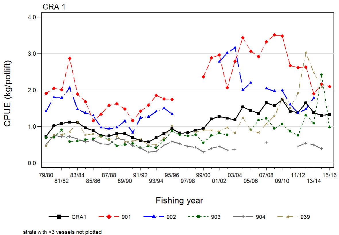
Figure 3: Arithmetic CPUE for CRA 1 by fishing year and statistical area from 1979–80 to 2015–16. This figure generated from data prepared using the F2 algorithm scaled to the combined “LFX” destination codes.
