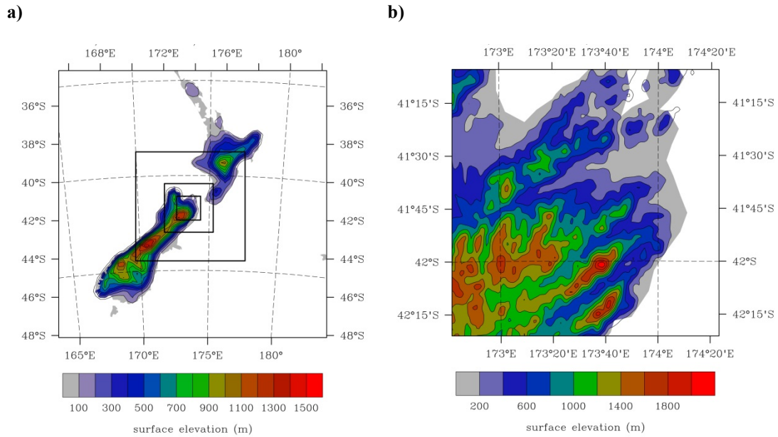
Figure 2: Weather Research and Forecasting model nested grid configuration, showing terrain height, a) for all four grid domains, and b) the high-resolution domain (grid 4).
