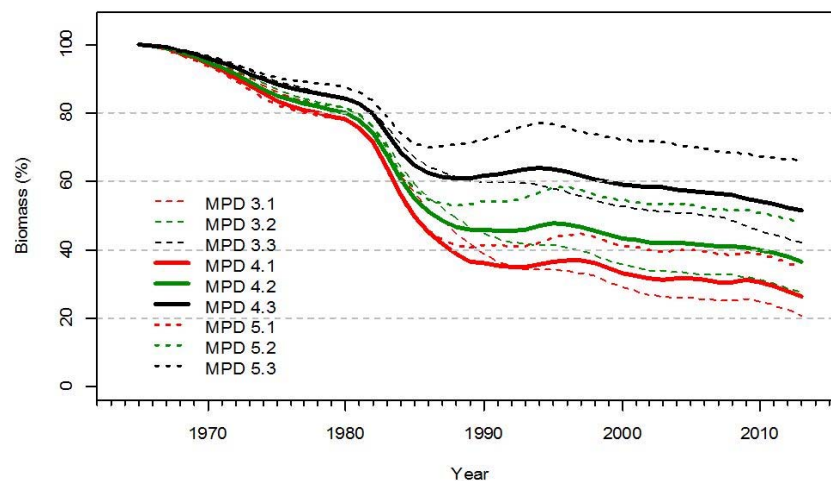
Figure 5: Top: Estimates of spawning stock biomass for MPD models 3.1, 3.2, 3.3, 4.1, 4.2, 4.3, 5.1, 5.2, and 5.3. Bottom: Estimates of spawning stock biomass as a ratio of B_0 (bottom panel) for MPD models 3.1, 3.2, 3.3, 4.1, 4.2, 4.3, 5.1, 5.2, and 5.3.
