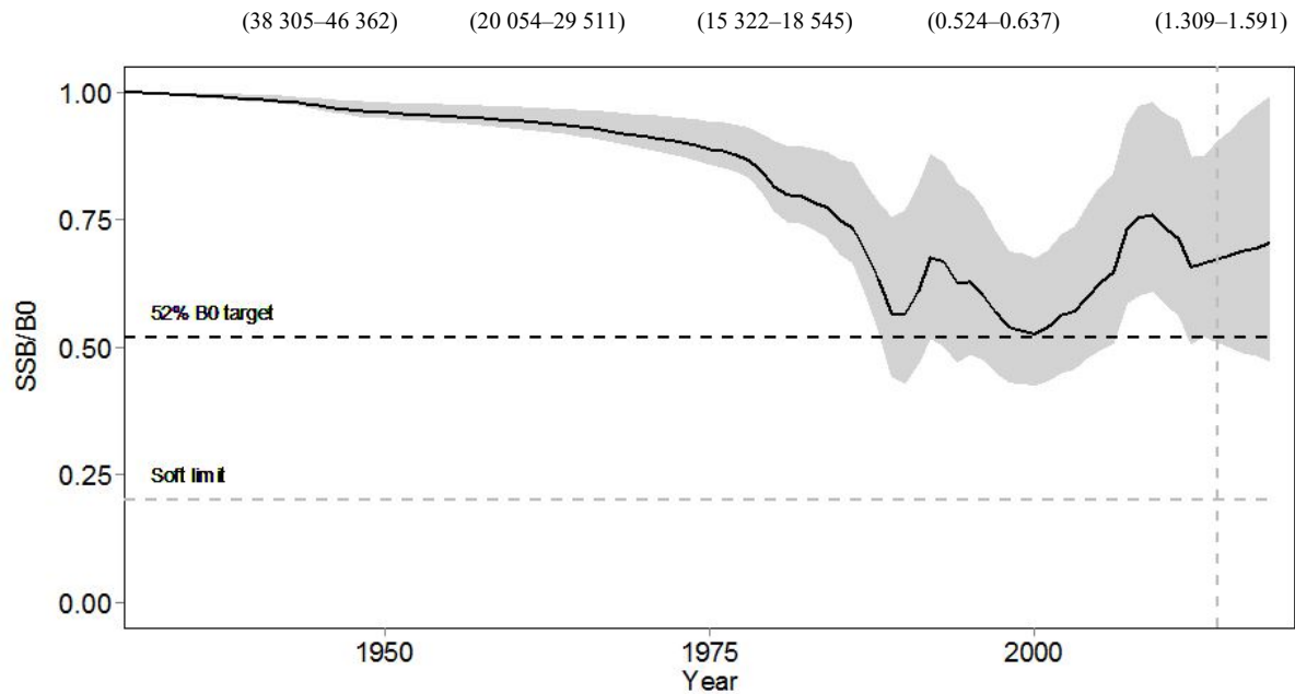
Figure 7: Spawning stock biomass relative to B_0 for the base model ( M = 0.20 , both abundance indices used; three chains combined). The 52% B_0 target set by the Minister of Fisheries in 2010 is denoted by a black dashed line and the 20% B_0 soft limit is denoted by the grey dashed line. The grey shaded area denotes 95% credible intervals derived from the MCMC model run and the black line denotes the median estimate for each year. The vertical dashed line denotes the first year of the projection period (2014).
