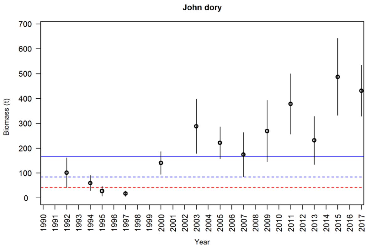
Biomass trends from the west coast South Island inshore trawl survey time series. Error bars are \pm two standard deviations. The solid blue line represents the interim target and dashed blue and red lines the soft and hard limits, respectively.
