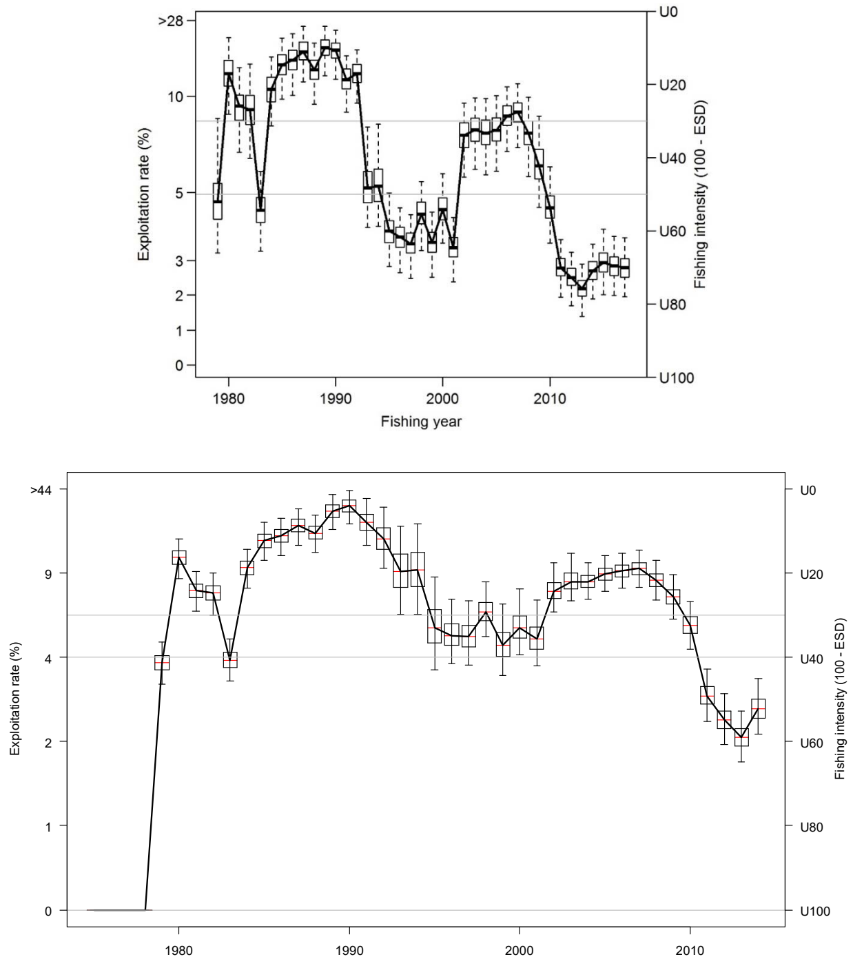
Figure 19: ESCR base, MCMC estimated fishing-intensity trajectory. The box in each year covers 50% of the distribution and the whiskers extend to 95% of the distribution. The fishing-intensity range associated with the biomass target of 30–50% B_0 is marked by horizontal lines.
